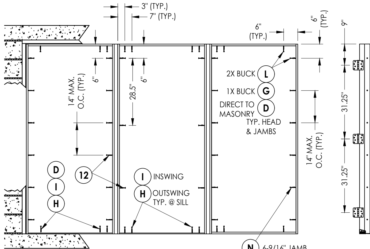
FRAME ANCHORING
