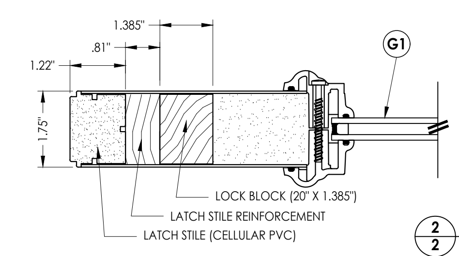
2 2 HORIZONTAL CROSS SECTION
